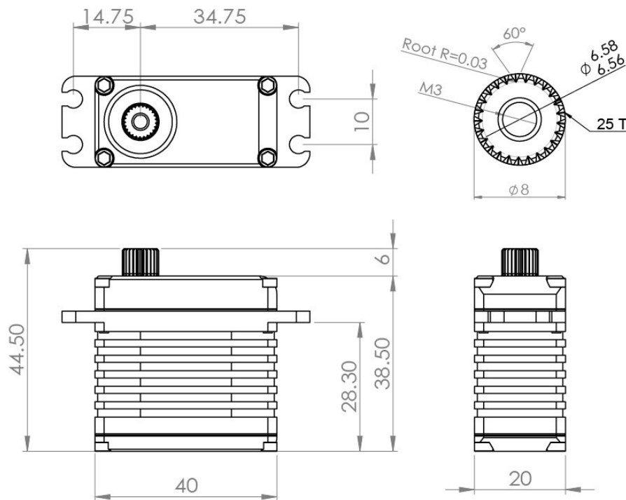
Figure 1: CBS-20 dimensions.
