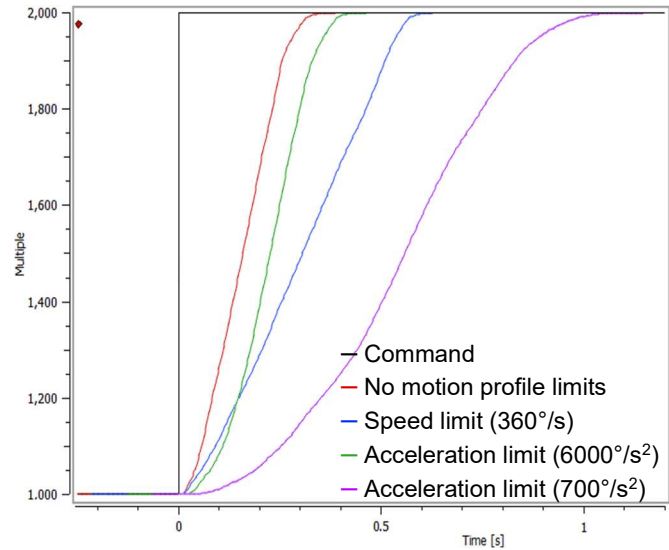
Figure 2: Servo position step response with different motion control profiles.
